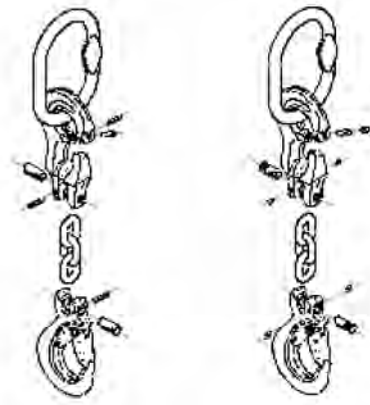
DISMOUNTABLE CONNECTIONS
